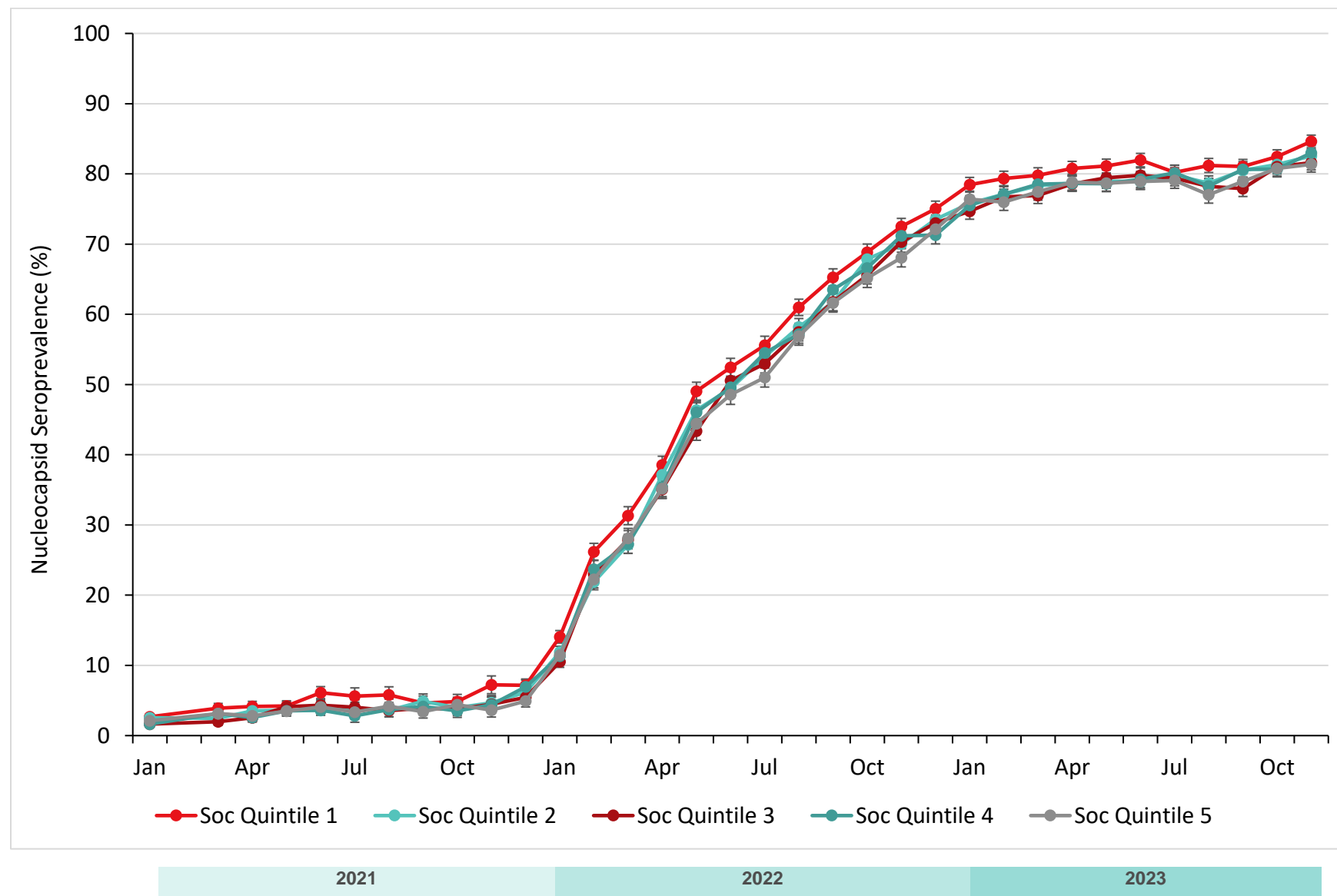
Figure 5D. Temporal trends of SARS-CoV-2 seroprevalence by monthly intervals from January 2021 – November 2023 estimated by Nucleocapsid antibody results by social deprivation level (1 = least deprived and 5 = most deprived).
