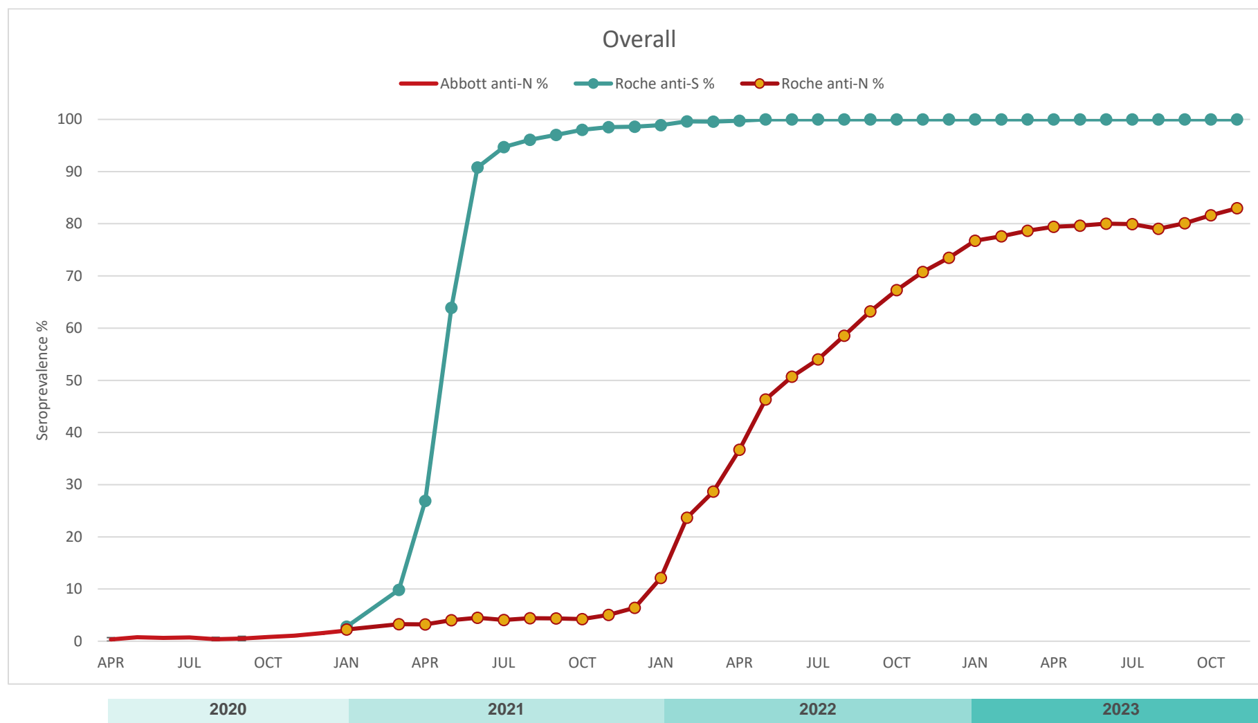
Figure 1. Overall temporal trends of SARS-CoV-2 seroprevalence by monthly intervals from April 2020 - November 2023 (comparing results from Abbott anti-N (until January 2021) followed by seroprevalence estimated by Roche anti-N and Roche anti-S results).
