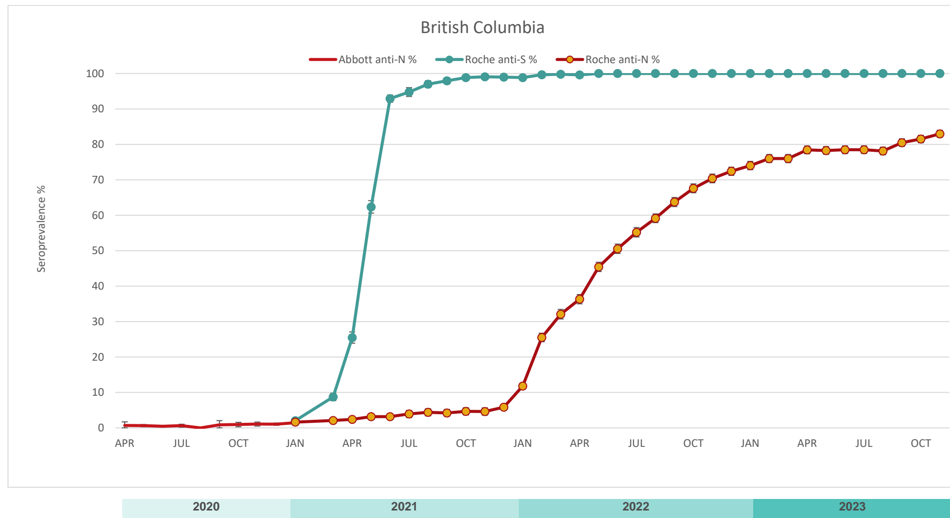
Figure 2. Regional temporal trends of SARS-CoV-2 seroprevalence monthly from April 2020 – November 2023 (by Abbott anti-N, Roche anti-N and Roche anti-S assays)
