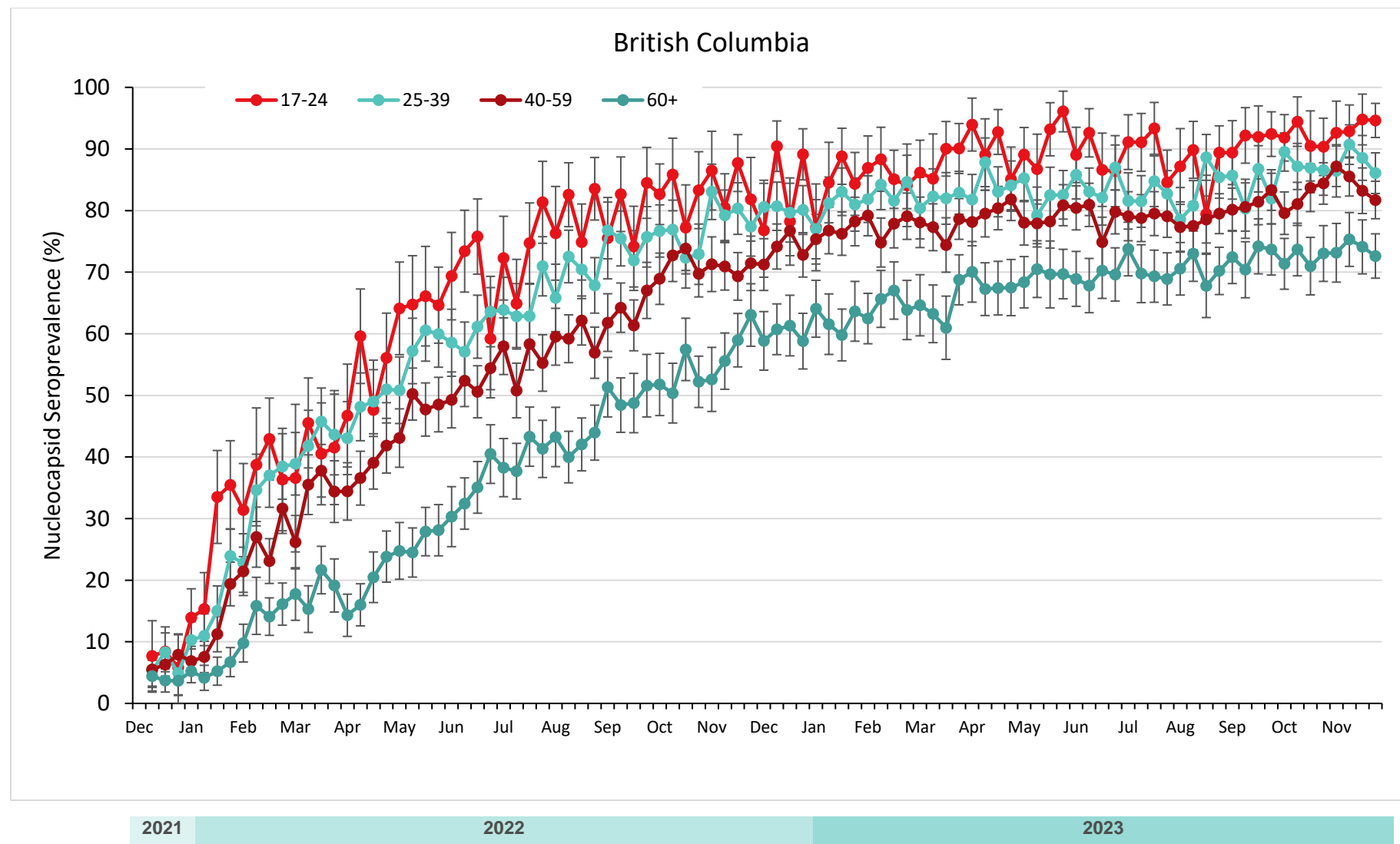
Figure 4. Regional temporal trends of SARS-CoV-2 Nucleocapsid (infection) seroprevalence by age group weekly from December 2021 – November 2023
